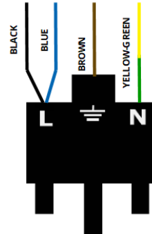
PROMATIC DURAPLUG
