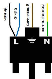
PROMATIC DURAPLUG
