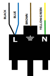
PROMATIC DURAPLUG
